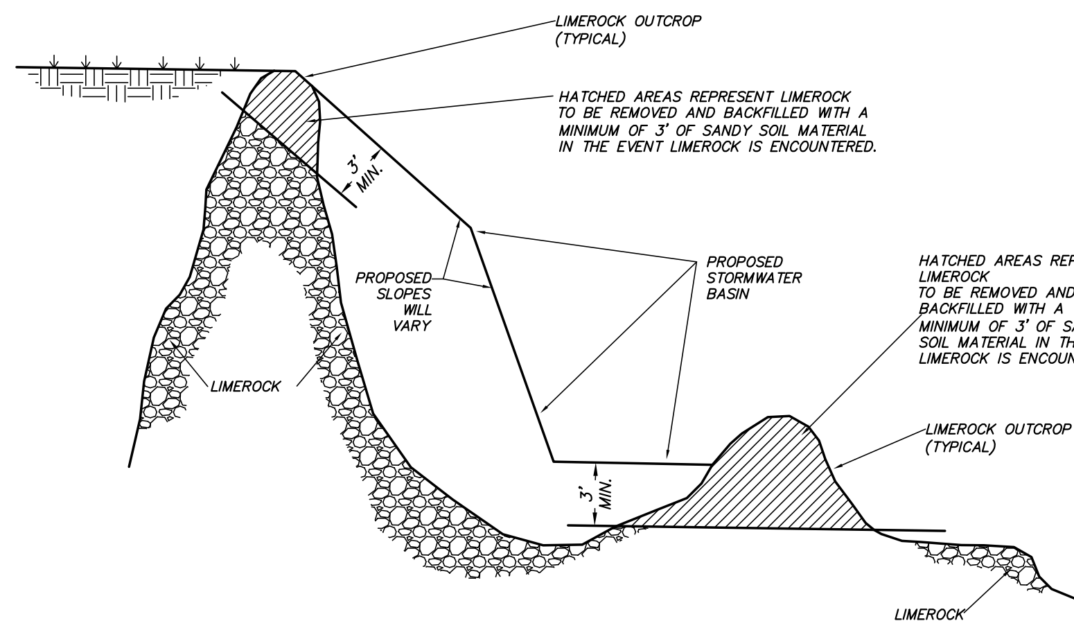
LIMEROCK OUTCROP REMOVAL DETAIL NTS
