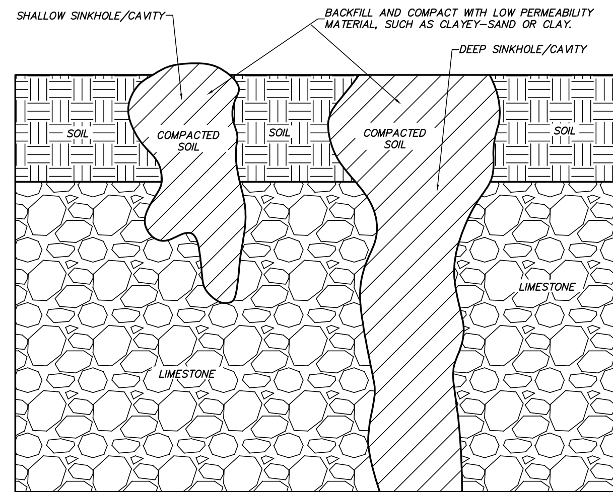
SHALLOW AND DEEP SINKHOLE/CAVITY MAINTENANCE REPAIR DETAIL NTS
